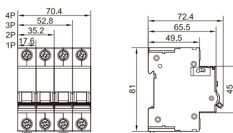
BHD20/40/80
