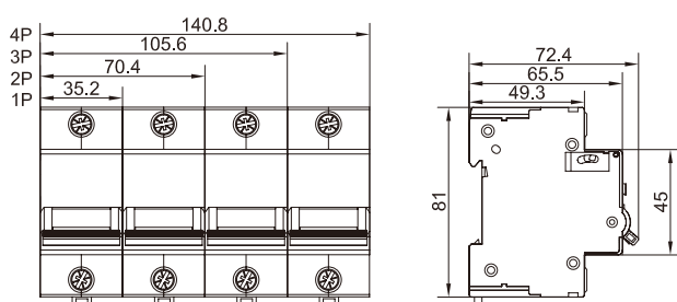
BHD120/250
